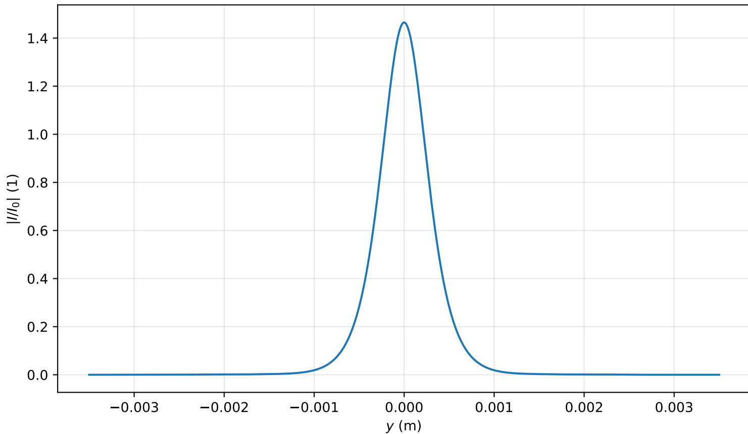
Intensity profile I(x=0, y, z=3.662)/I_0 , \text{Pin}=0.9\text{Pcr} , artificial time
